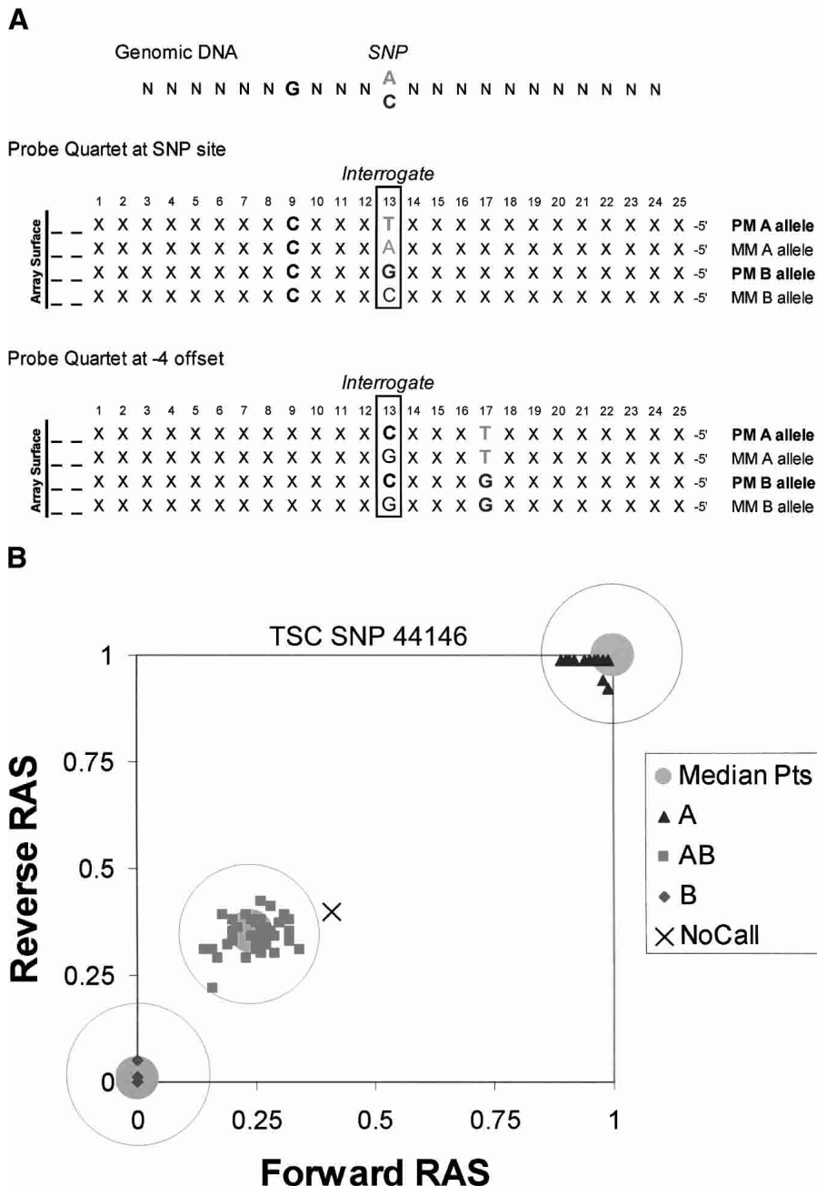
Figure 2 (A) Sequence prototypes of the oligonucleotide probes. Twenty-five-mer oligonucleotides which are complementary to SNP sites and flanking sequences are synthesized on the surface of the array. The 13th nucleotide is the interrogative position where the probe sequences are either perfectly matched (PM) or mismatched (MM) to one of the two alleles of the SNP. The PM and MM probe pairs provide a basis for signal vs. noise measurements. The two probe pairs corresponding to the two alleles are grouped as probe quartets. Shown are the prototype sequences of the probe quartet at the SNP site, where the probe sequences differ only at the SNP site which is also the interrogative position. To provide data redundancy, four additional probe quartets are offset from the SNP site by one to four nucleotides in either direction. Also shown are prototype sequences for the probe quartet offset by -4. In this offset probe quartet, the SNP site has shifted to position 17 of the 25-mer. The probe sequences in this quartet are different at -4 (PM vs. MM) and at the SNP site (allele A vs. B). Each SNP is represented by five probe quartets (one at the SNP site and four offset) in both orientations, for a total of 40 oligonucleotide probes. (B) Genotype calling. The RAS is a measure of the signal intensities contributed from the A allele compared to signals from both alleles. Median RAS values from forward and reverse probe quartets define points in x - y coordinates. RAS points from the algorithm training set of 133 ethnically diverse individuals were clustered to determine the three median points, shown as large gray points. Genotypes are assigned for each SNP by determining the shortest distance between RAS points and one of the three median points. Call zones are drawn around the median points to increase the stringency of the genotype assignments. Shown are the RAS points from 99 individuals in 33 CEPH trios for TSC SNP 44146. One of the individuals was not assigned a genotype because the RAS point fell just outside the AB call zone.
